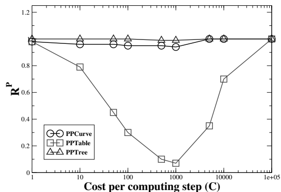
Figure 5: Performance of the different performance profiles in the scheduling domain. Values closer to 1.0 are better. PPTree outperforms both PPTable and PPCurve.
